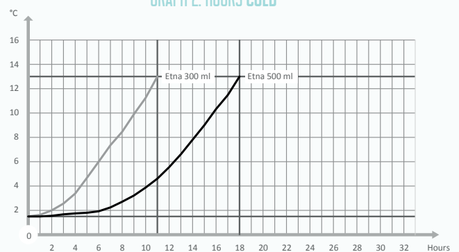
GRAPH 2: HOURS COLD
